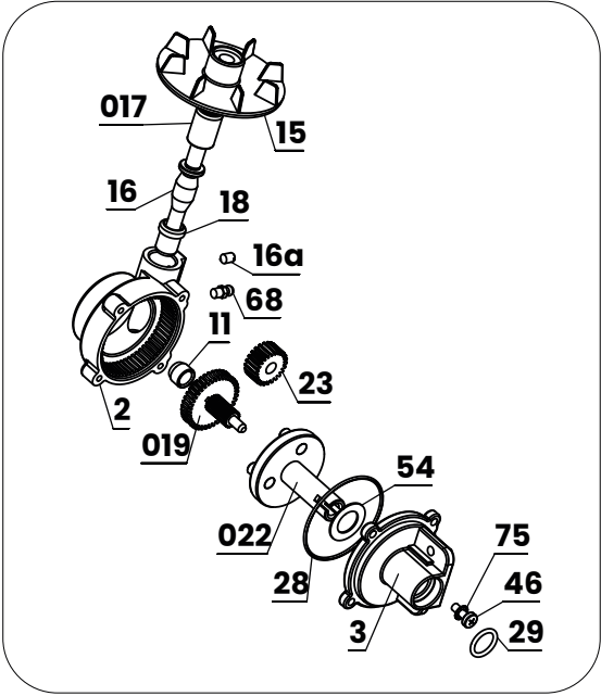
Pos. 02 10148 Complete gearbox - Slow 10170 Complete gearbox - Fast
