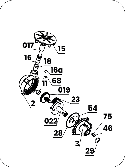
Pos. 02 10597 Complete gearbox - Slow 10795 Complete gearbox - Fast
